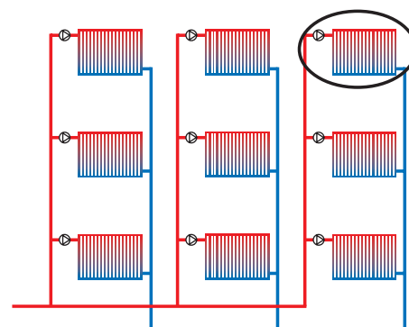
Fig. 6: Measure on the last radiator (valve).
